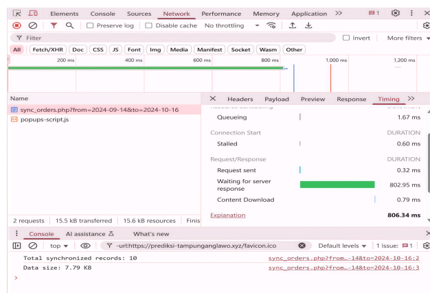
Figure 8. Data synchronization via API
