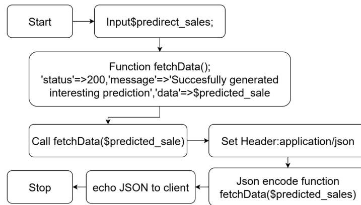
Figure 4. API flowchart for the prediction system
