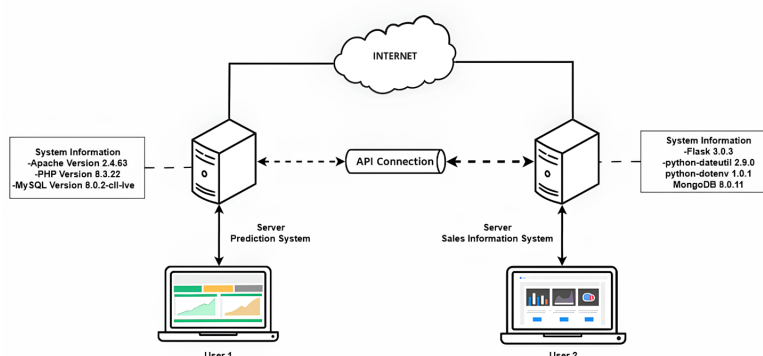
Figure 7. System testing topology scheme
