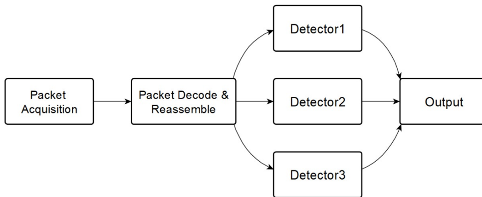
Figure 3. Architecture of Packet Processing Suricata
