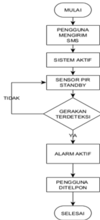
Figure 2. System Flowchart
