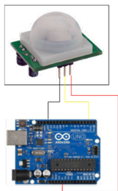
Figure 3. Connecting Sensors with Arduino
