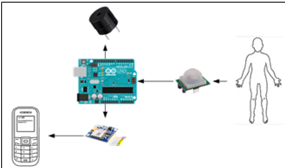
Figure 1. Block Diagram
