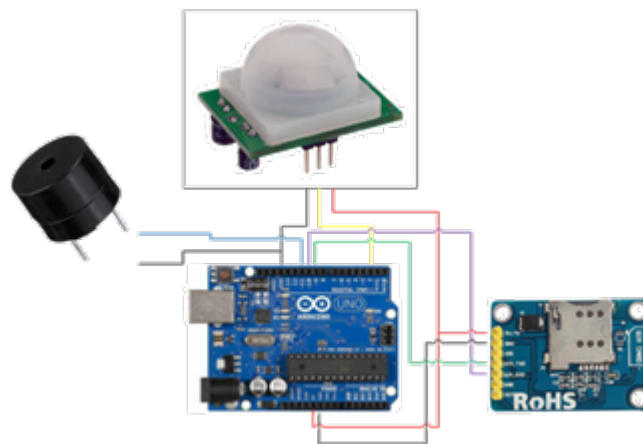
Figure 5. Connect the PIR Sensor, Buzzer and GSM module
